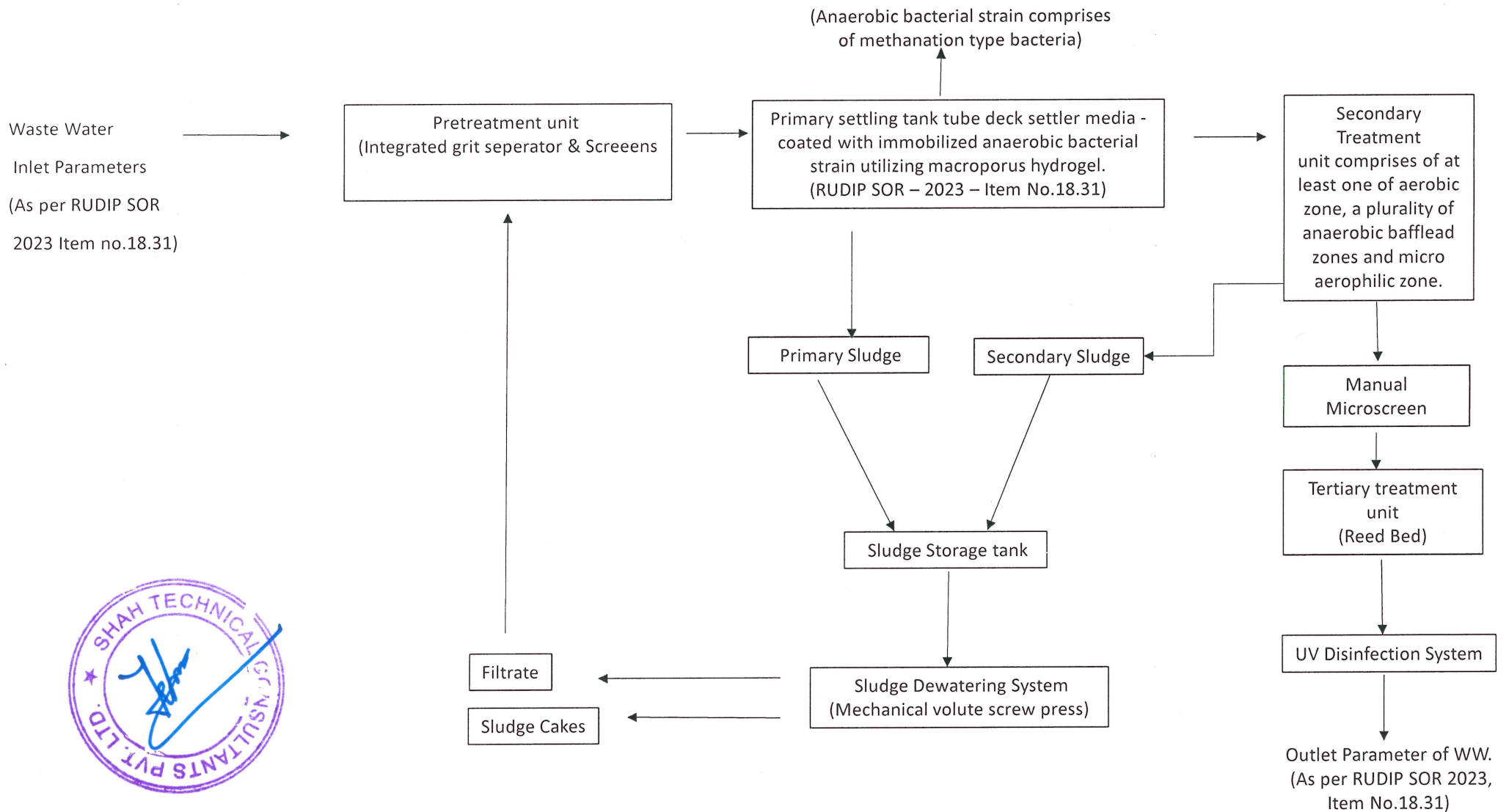
Flow Diagram For Treatment Process Of RUDIP-WWTP
